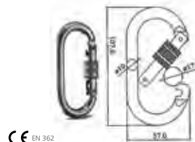
LX03 Carabiner/ Screw Gate Alloy Steel. MBL: 22kn
