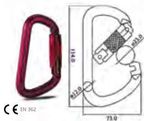
LX08 Carabiner / Triple Lock Aluminium Alloy MBL: 25kn
