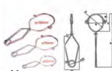
LX06 Pipeform Anchor Stainless Steel Wire Size: 2" / 3" / 4" MBL: 27kn
